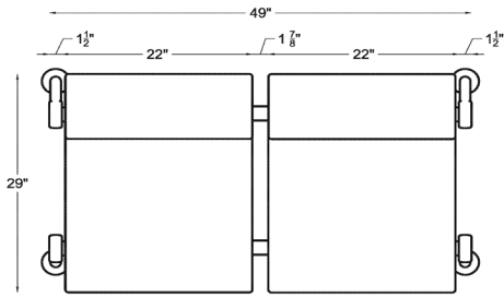
ex. 1 : Two seat unit with gap. Beam length 49" / 1245 mm.
